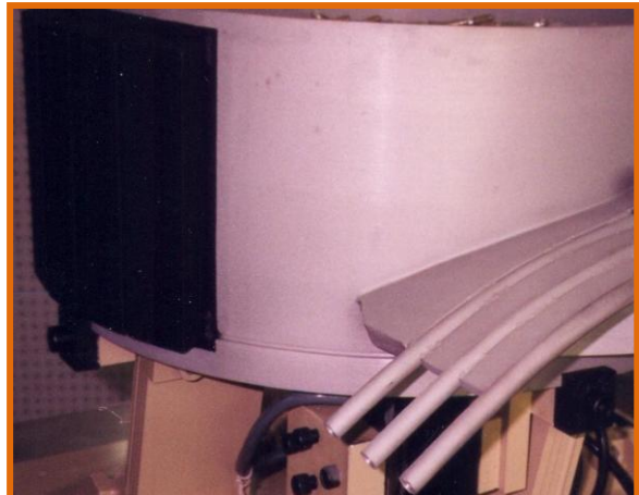
Single lane feeding for better orientation of cylinder and spherical parts.
