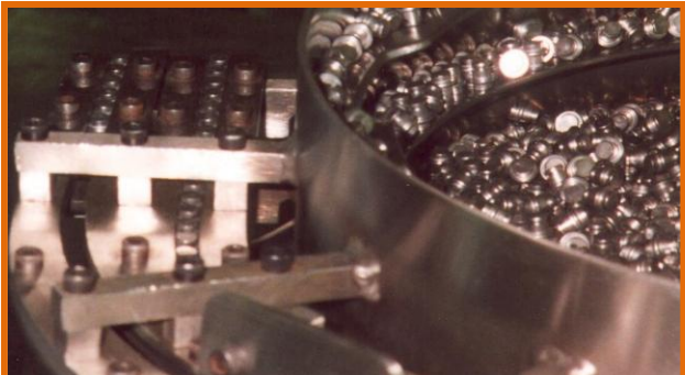
Multi-laning out of the bowl will provide a smaller loading platform.
